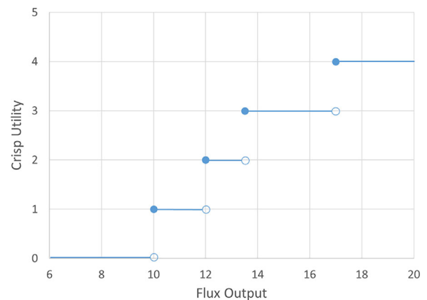
FIGURE 5 Crisp utility score for every possible threshold met for flux output
