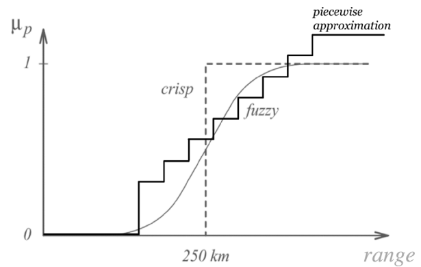
FIGURE 2 Plot of preference for a product (from 0 to 1) versus the desired range. Dotted line represents the crisp number and solid line represents the fuzzy number. Darker solid line represents piecewise linear approximation of fuzzy number
