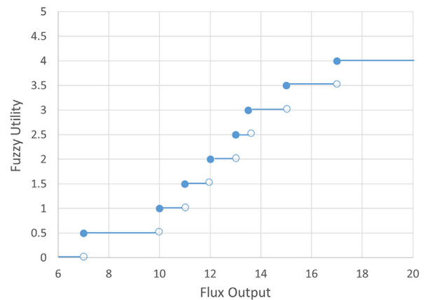
FIGURE 7 Fuzzy utility function which approximates fuzzy numbers with a piece-wise linear function. Example is shown for flux output
