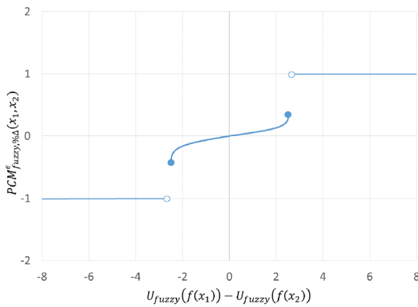
FIGURE 10 Possible values for the fuzzy percent change pairwise comparison matrix given two devices
